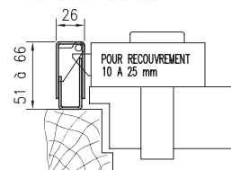
GACHE A DECALAGE REGLABLE
